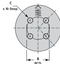
ISNG 1500 TO ISNG 7500 STYLE CYLINDER
